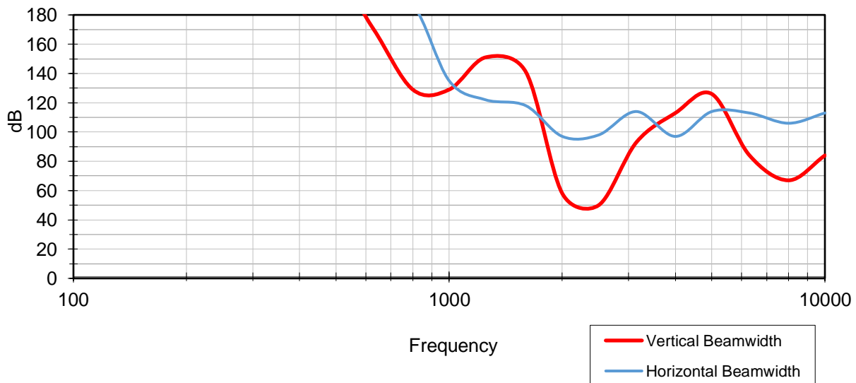
106/HTH @ 6dB down
