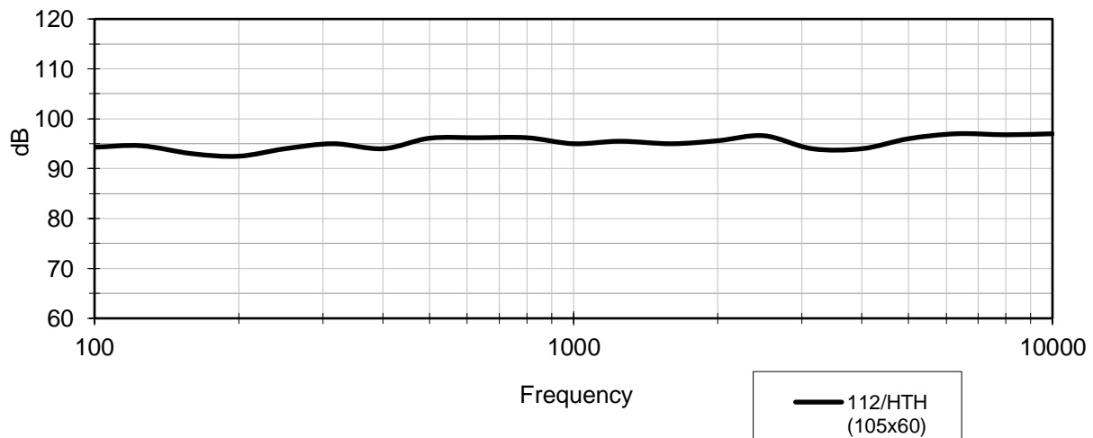
Frequency Response: 112/HTH (105x60)
