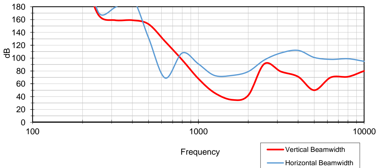
112/HTH (105x60) @ 6dB down
