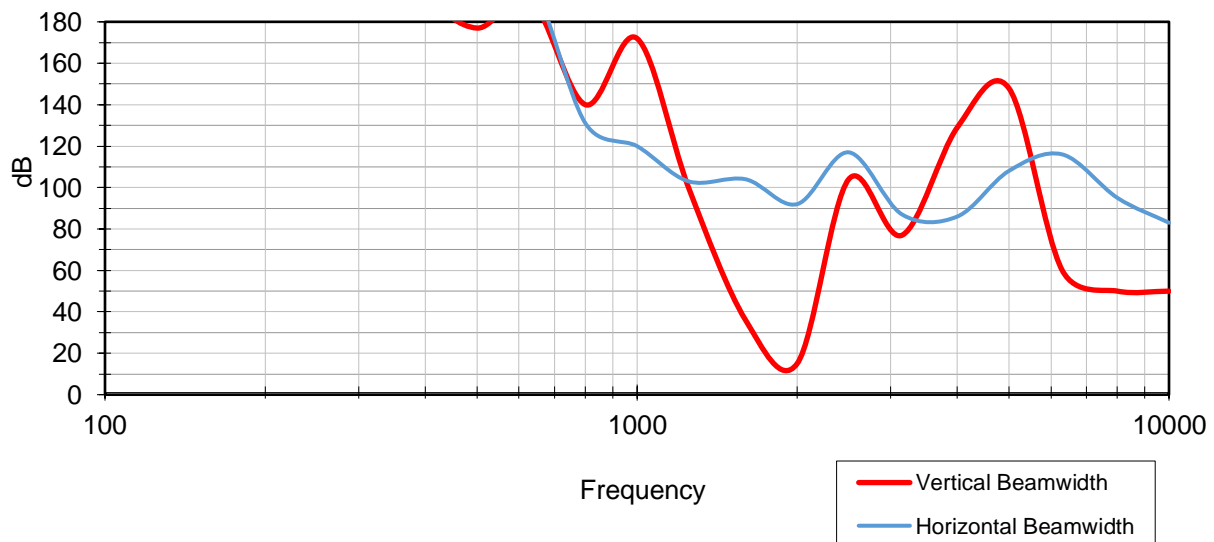
108/STC @ 6dB down
