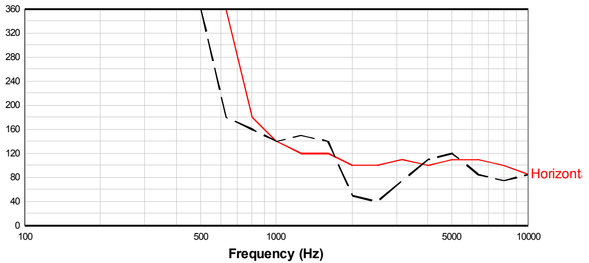
Beamwidth versus Frequency 106IM
