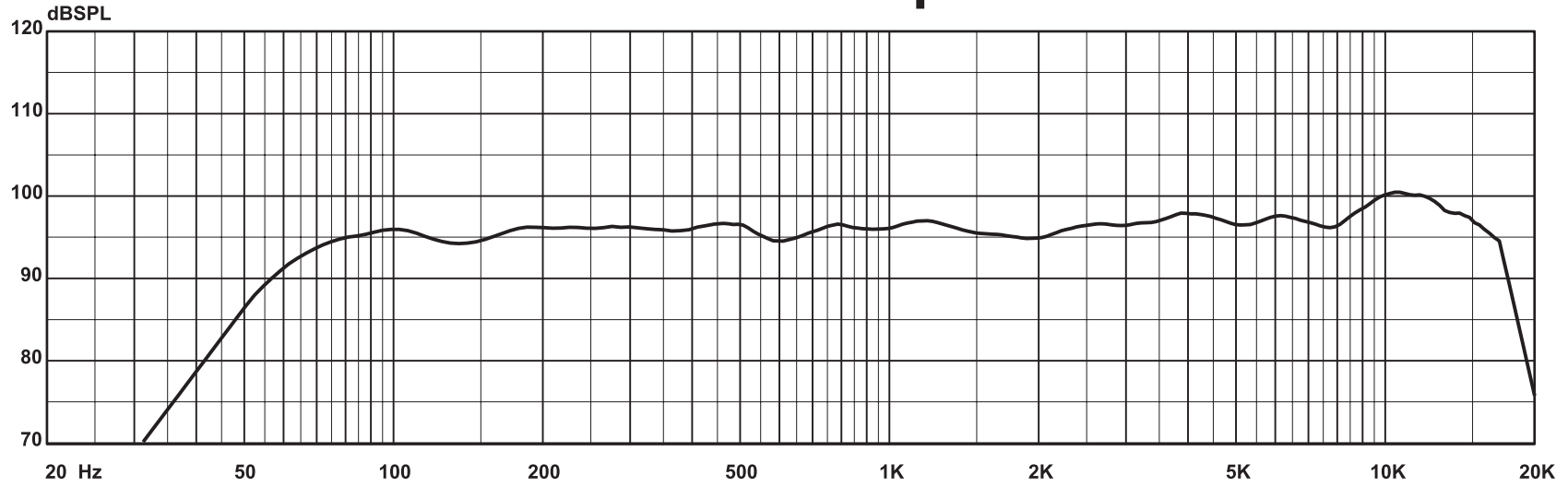
115TW 105x60 Active
