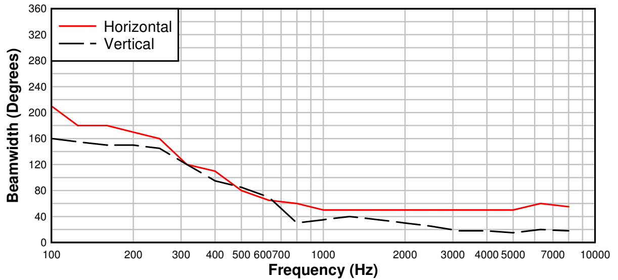
Beamwidth versus Frequency Cross Field Array
