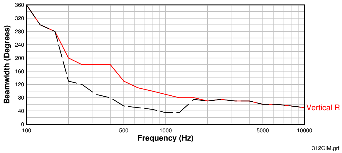
Beamwidth versus Frequency 312CIM
