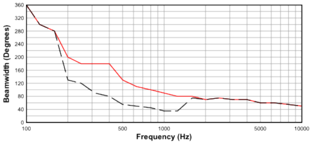
Beamwidth versus Frequency 312CIM (Vertical Black Horizontal Red)
