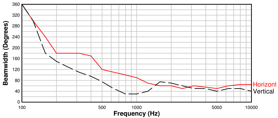
Beamwidth versus Frequency 112IM 60 X 40 Active
