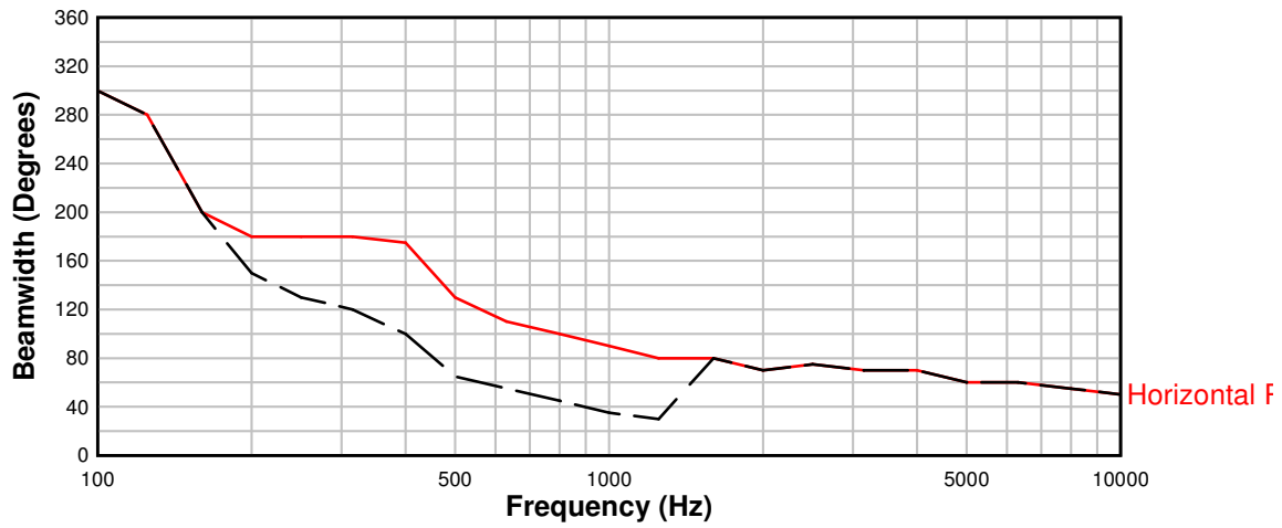
Beamwidth versus Frequency 212CIM
