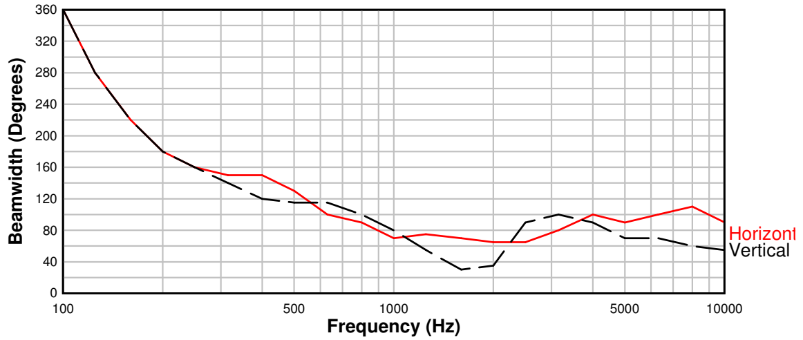
Beamwidth versus Frequency 115UM 105 x 60
