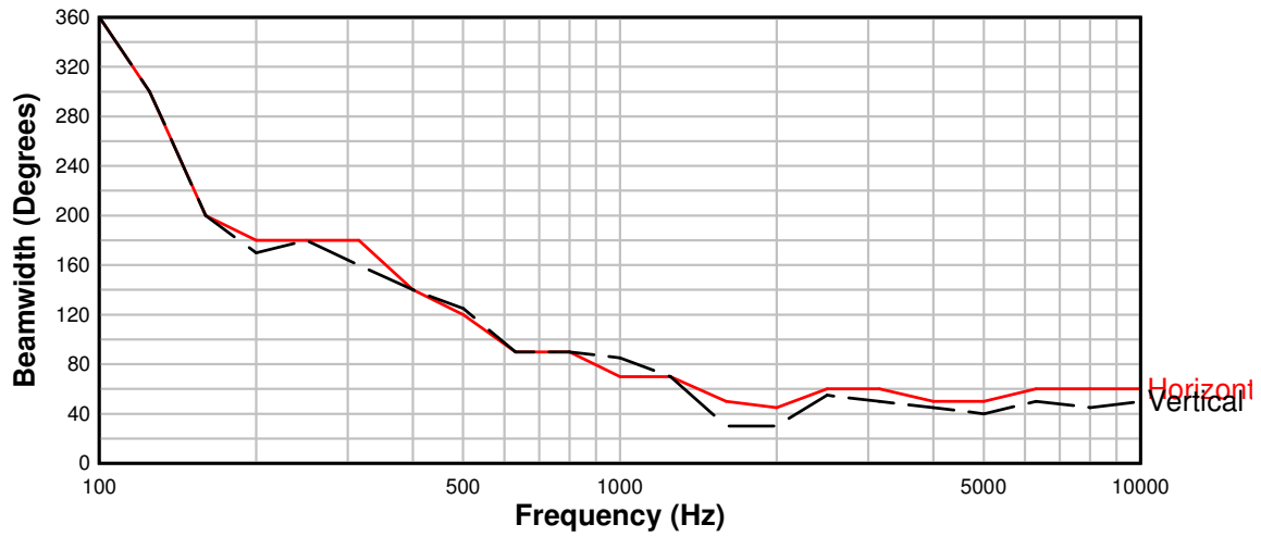
Beamwidth versus Frequency 115TW 60 X 40
