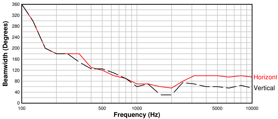
Beamwidth versus Frequency 115RW 105 X 60
