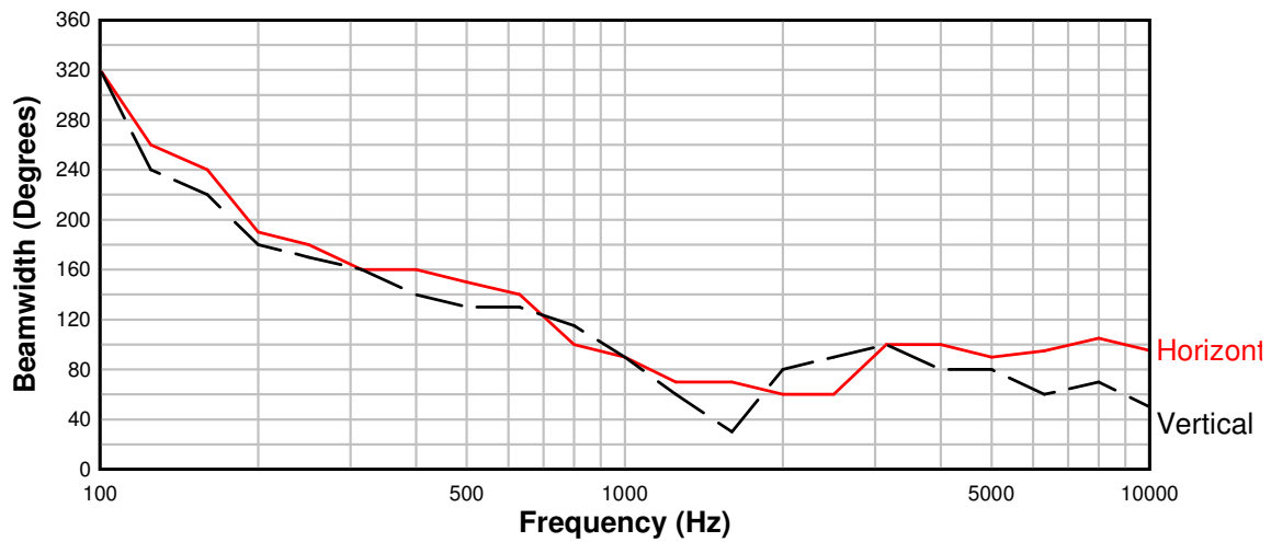
Beamwidth versus Frequency 112UM 105 X 60
