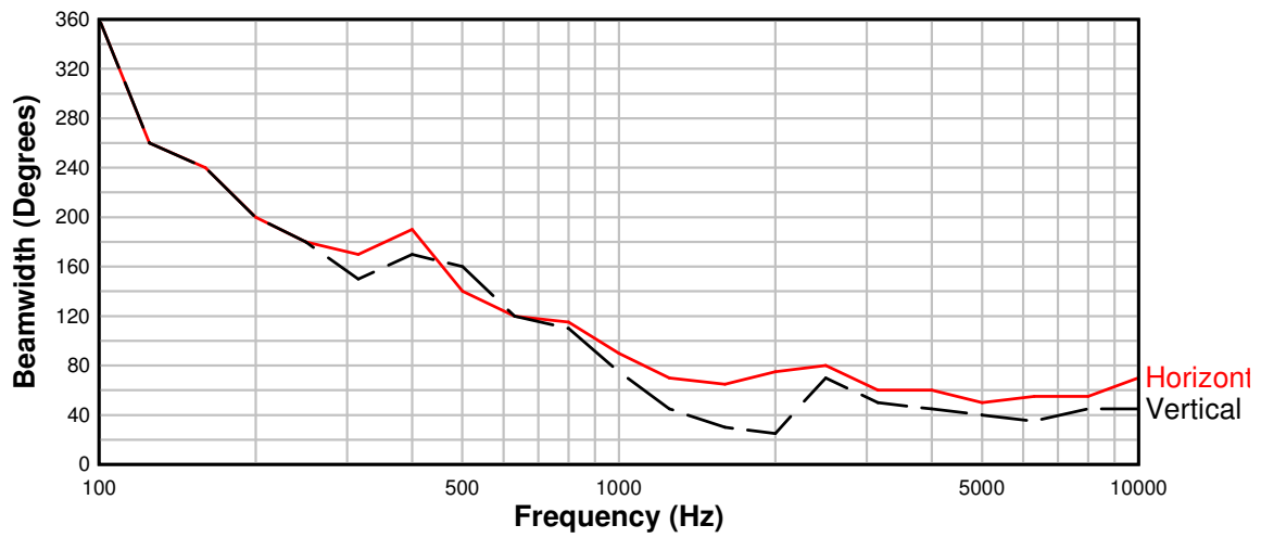
Beamwidth versus Frequency 112IM 60 X 40
