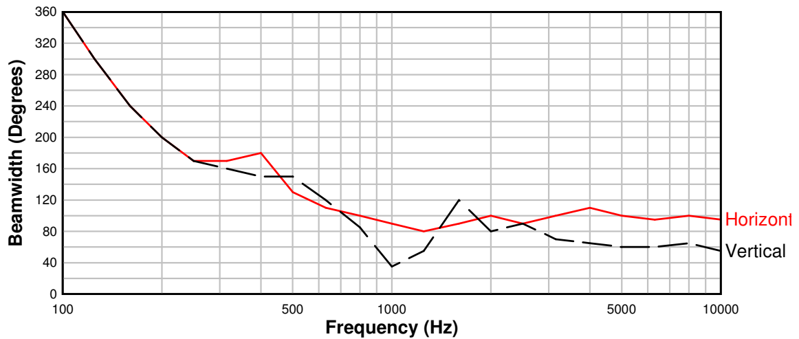
Beamwidth versus Frequency 112IM 105 X 60 Active
